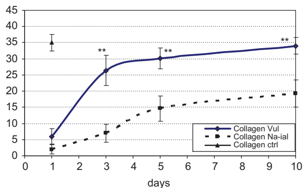
Figure 5. Percentage of wound area filled with thin orange/yellow-green collagen fibers in Vulnamin (bold line) and Na-lal (dotted line) treated wounds according to days post-wounding. ** p < 0.01 .
